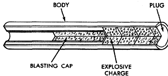
Fig 5-12 BOMB BURSTER, C8R1
